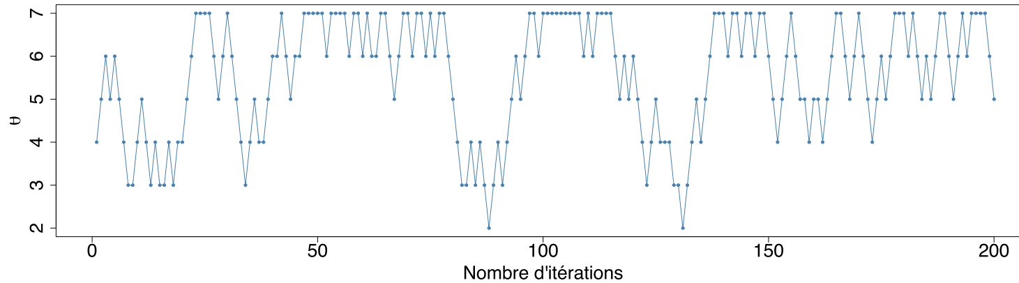
Algorithme Metropolis
